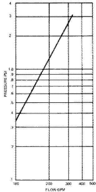
PRESSURE LOSS F429 ADAPTOR F214B, FLOW IN EITHER DIRECTION.
