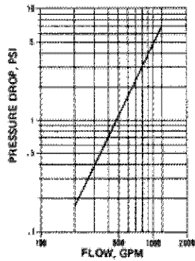
PRESSURE DROP VS FLOWRATE LOADING CONNECTIONS
